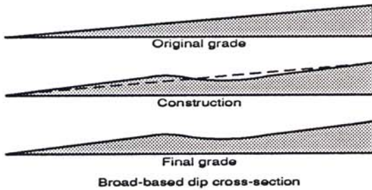
Figure 6. Broad-based dip.
