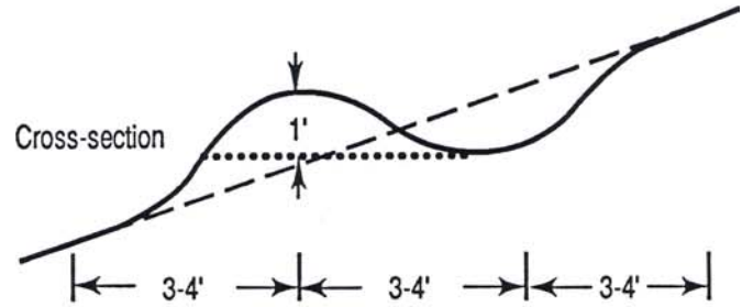
Figure 7. Water bar.
