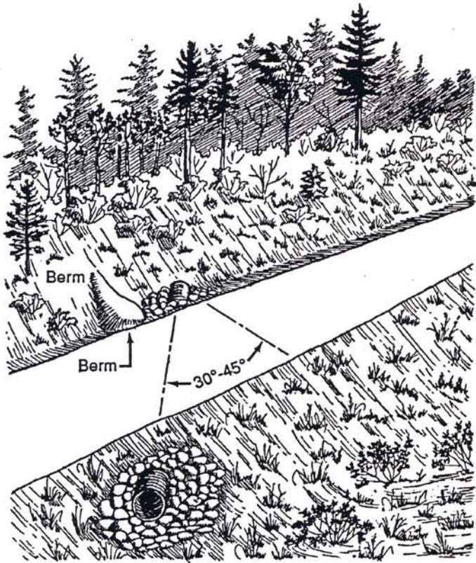
Figure 5. Cross-drain culvert.
